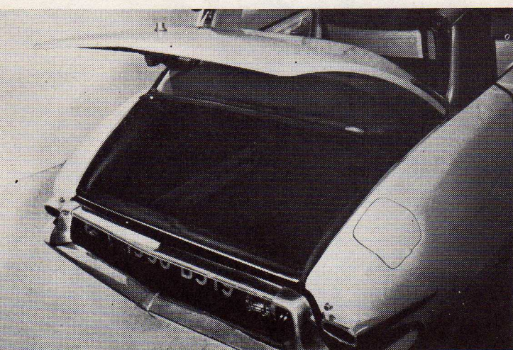
With the spare wheel conveniently carried in the front, and the fuel tank rectangular in shape and pushed well forward, the trunk space becomes unusually deep.
