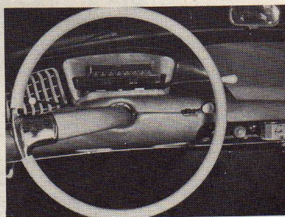
LEFT: Front suspension and drive of the Citroën. Articulating arms are set well back of drive shafts in roller mounts. RIGHT: One-spoked wheel & dash panel.
